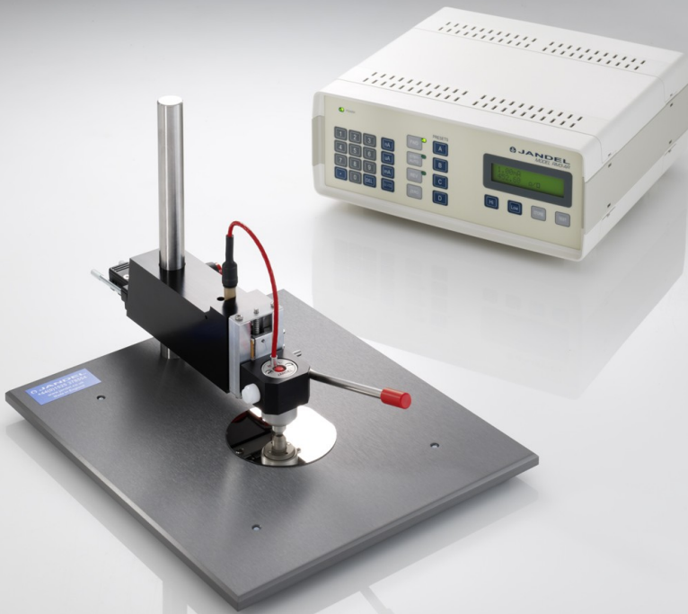
Multi Height Probe with Arm Lowered for Measuring a Flat Material
